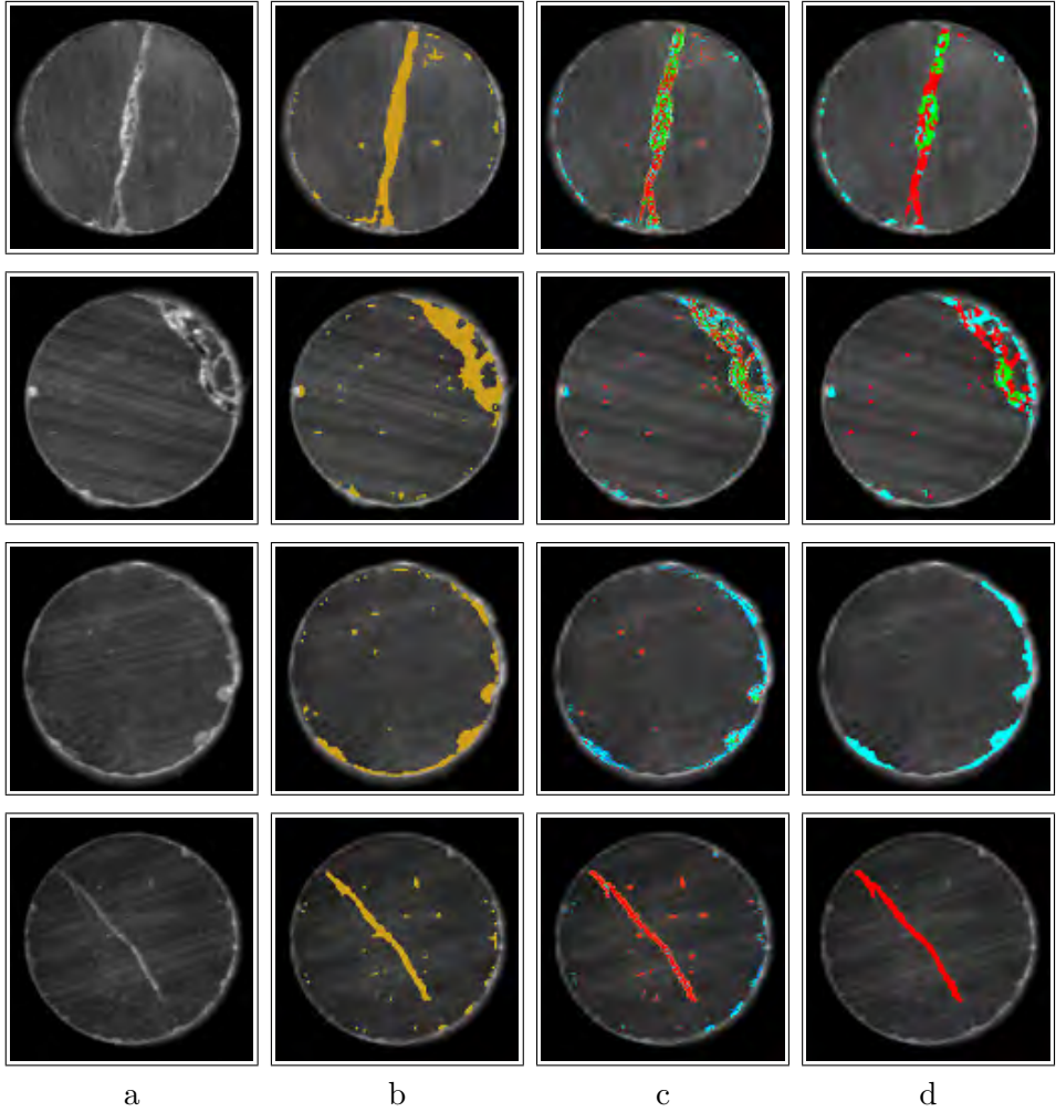
FIGURE 23. Cylindrical magnets II, diameter 10 mm. Magnification: 0.057 mm/pixel. 4279 training patterns, 14 classes, 64 features. From top to bottom: four examples. a: Source images. b: Detected irregular regions. c: Raw classification results. d: Postprocessed classification results.
