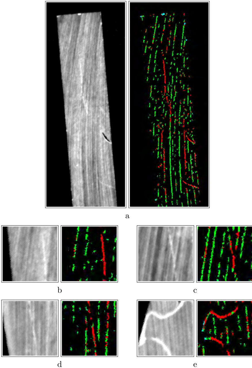
FIGURE 19. Example of the limits of the method: classification of the irregular regions into two classes: grooves from grinding (green) and cracks (red). Small chips (blue) also visible. a: Source and classification result of the whole image. b-e: details of this and other images.
