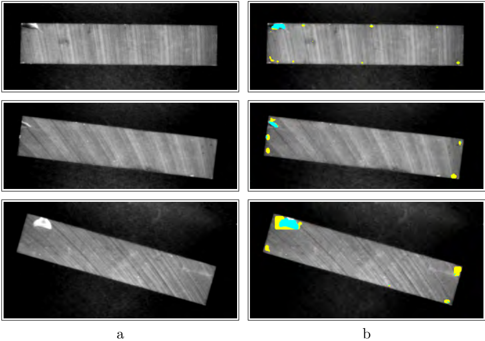
FIGURE 22. Plate magnets, dimensions 60*12 mm. Magnification: 0.15 mm/pix. 2257 training patterns, 10 classes, 44 features. Object occupies approx. 400*80 pixels. From top to bottom: three examples. a: Source images. b: Postprocessed classification result.
