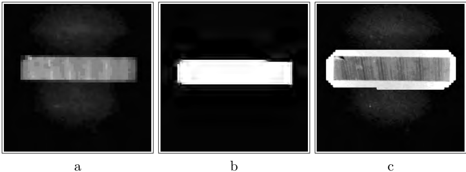
FIGURE 8. Finding the approximate background. a: Image of Fig. 7a scaled down – brightness of background spots reduced. b: Image a thresholded with the same threshold as in Fig. 7b. c: Result: image b scaled back and dilated (original object overlaid only for comparison).
