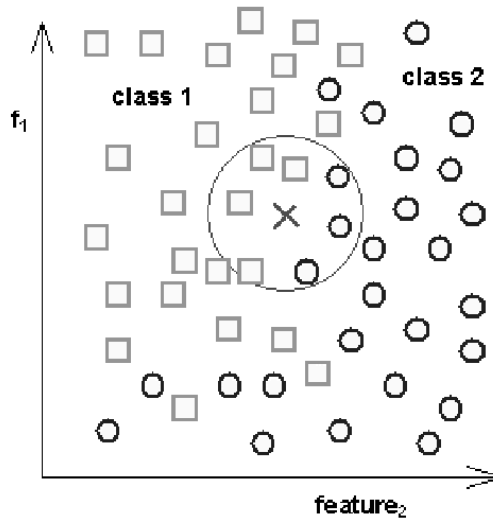
FIGURE 12. The basis of the k nearest neighbours classification – the case of k = 7 . The unknown object (cross) is classified as belonging to the class 1 (squares), because among its 7 nearest neighbours the majority belongs to that class.
