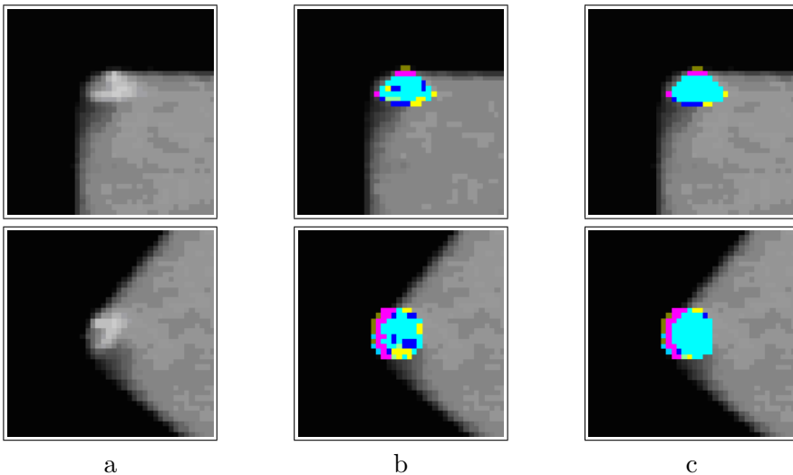
FIGURE 17. Generalisation power of the classifier and invariance to rotation and shift of the tested object. Upper row: object in position I; lower row: the same object in position II. a: Originals. b: Classified with reduction of reference set. c: Postprocessed. Results for both positions do not differ significantly. (Figure belongs to section 10, page 221.)
