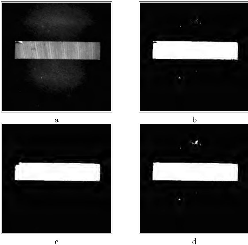
FIGURE 7. Contradictory actions of opening and closing. a: An object surrounded by dark region and some brighter spots far from the boundary. b: Image a thresholded: either parts of object left out or outer spots detected. c: Image b opened – background cleared, object incomplete (structuring element: 11 \times 11 round). d: Image b – object gaps filled in, background spots enlarged.
