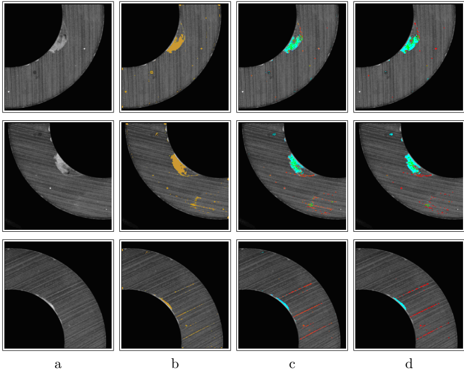
FIGURE 24. Loudspeaker magnets II, external diameter 50 mm. Same magnification and training as for cylindrical magnets of Fig. 20. From top to bottom: three examples. a: Source images. b: Detected irregular regions. c: Raw classification results. d: Postprocessed classification results. Note the problems with the grooves from grinding which seem as the cracks to the system. Upper and middle row show the different images of the same defect.
