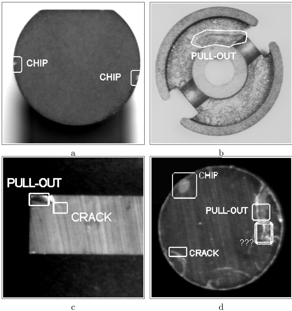
FIGURE 2. The most important surface defects. Chip – a and d; pull-out – b, c and d; crack – c and d. In c and d it can be seen how different types of defects can be difficult to classify univocally.
