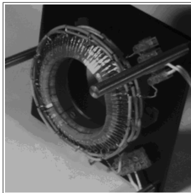
FIGURE 3. Double Layered LED Illuminator (DLEDI) – bottom view.
