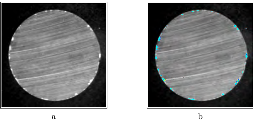
FIGURE 20. Cylindrical magnets I, diameter 37.5 mm. Magnification: 0.121 mm/pix. 681 training patterns, 8 classes, 44 features. a: Source image. b: Postprocessed classification result.
