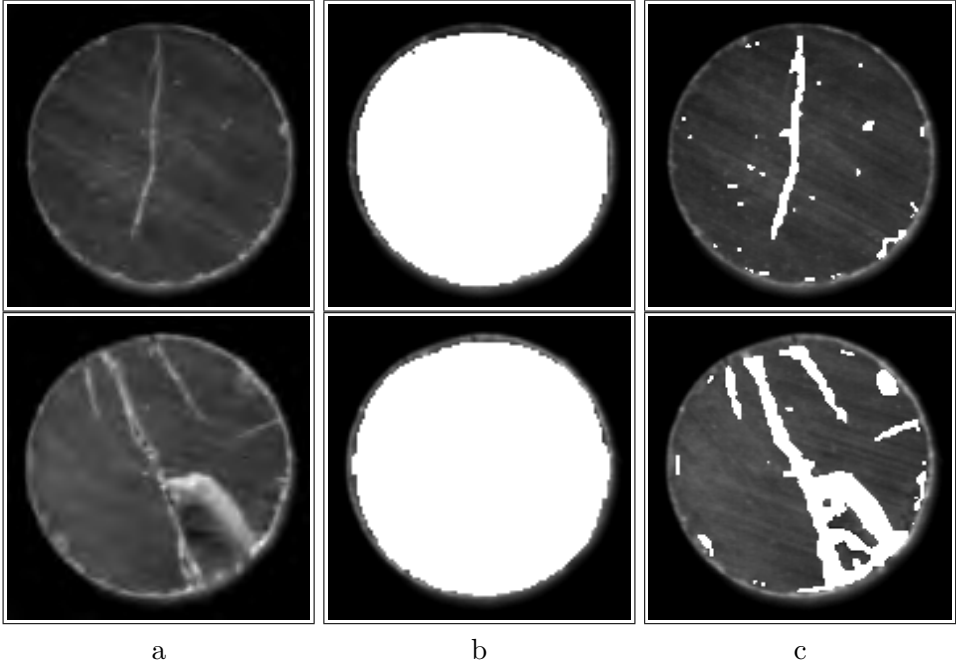
FIGURE 10. Detection of the region of interest (white) for defect classification – two examples (rows). a: Source images. b: Detected region of the object, as described in section 5.1 (narrow stripe at the object edge deliberately postponed). c: Regions with irregular brightness detected with the methods of mathematical morphology.
