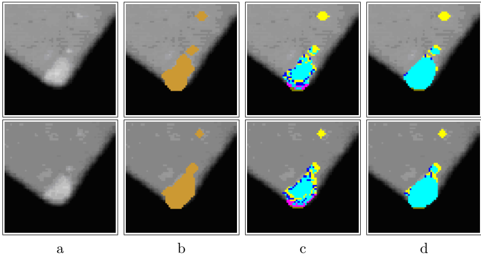
FIGURE 16. Generalisation power of the classifier and invariance to small lighting changes. Upper row: light I; lower row: light II. a: Originals. b: Detected irregular regions. c: Classified with reduction of reference set. d: Postprocessed. Results for light I and II do not differ significantly. (Figure belongs to section 10, page 221.)
